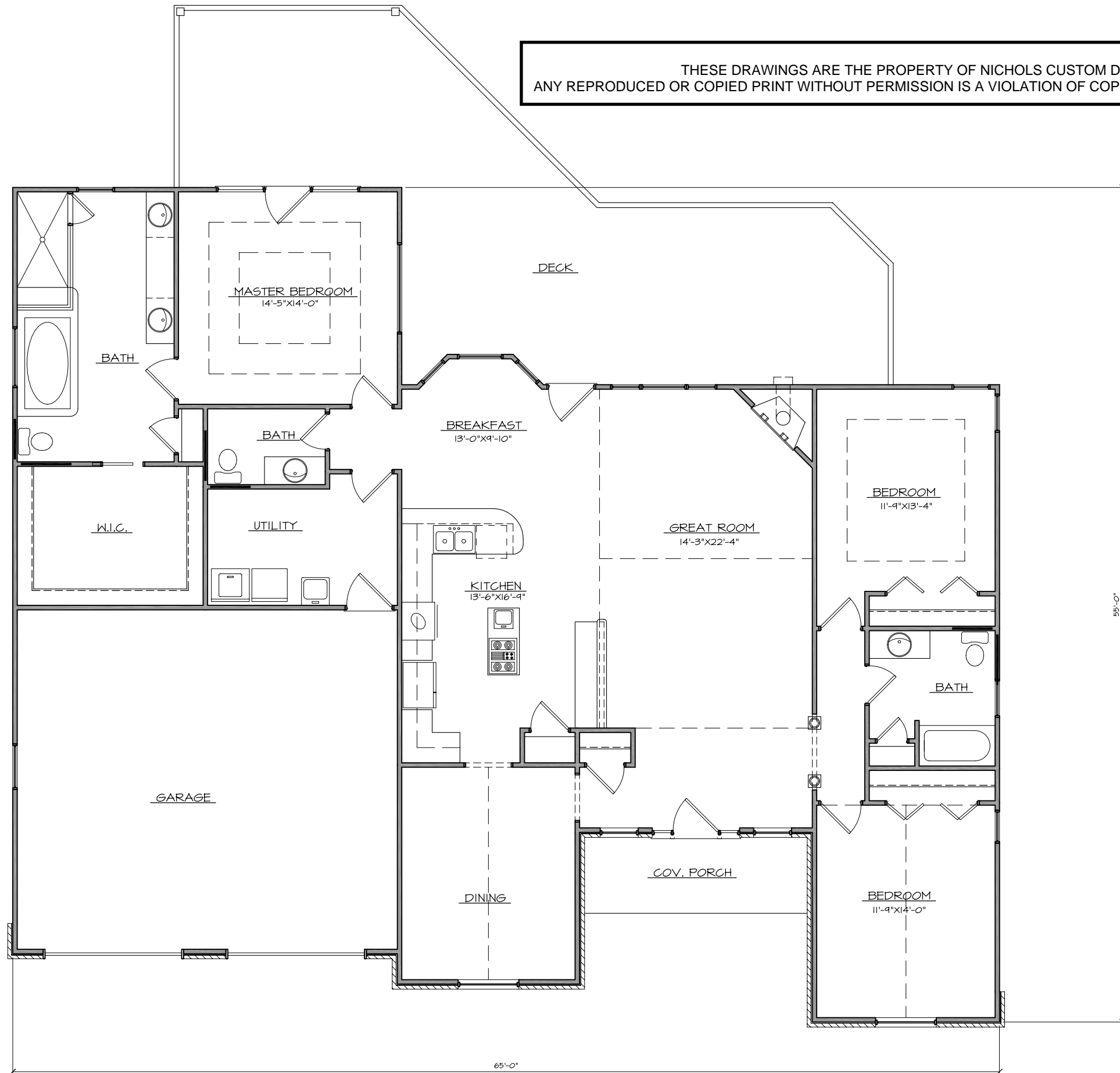
1 FIRST FLOOR PLAN A2 1/4" = 1'-0"
